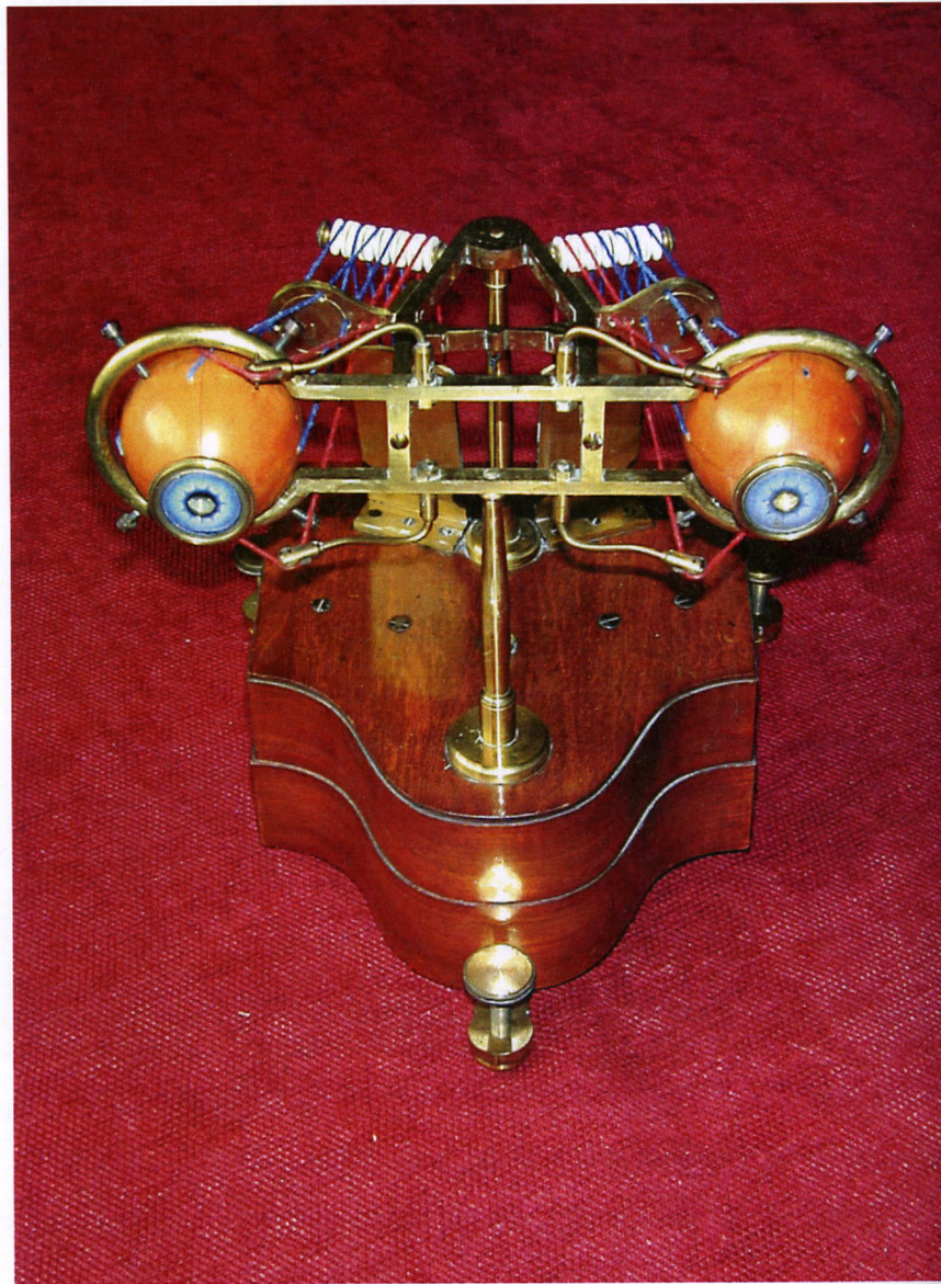
Fig.3 Ruete Ophthalmotrope
